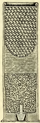
Green's Patent Swedish Cup Wad.
